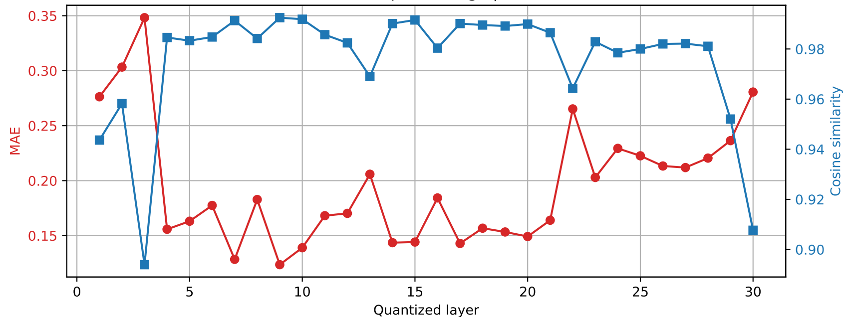
SmolLM2-360M | Prompt 1 Final RMSNorm output damage | float16 \rightarrow int4
