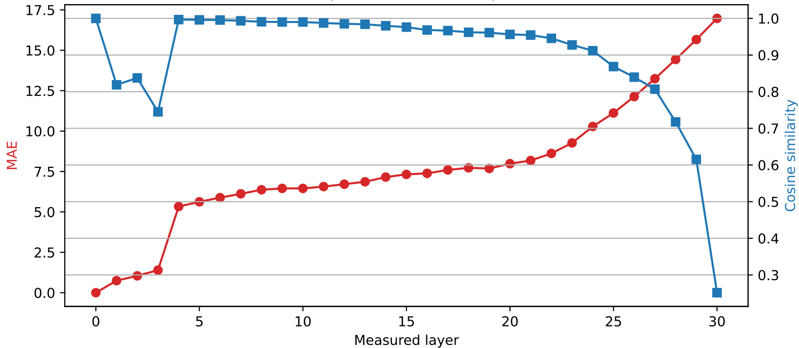
SmolLM2-360M | Quantized layer 0 | float16 → int4
