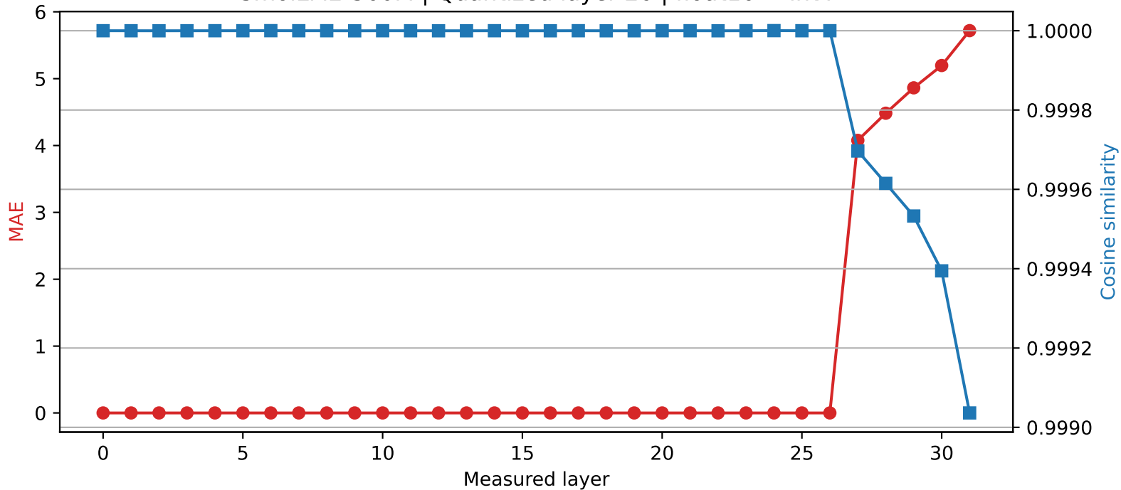
SmolLM2-360M | Quantized layer 26 | float16 \rightarrow int4
