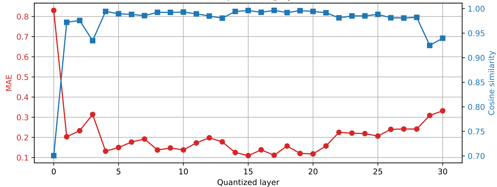
SmolLM2-360M | Prompt 2 Final RMSNorm output damage | float16 \rightarrow int4
