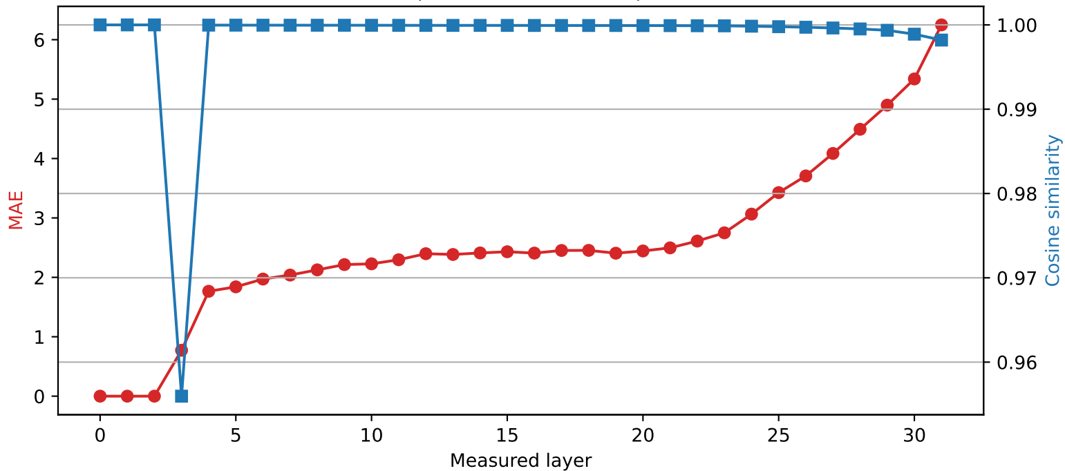
SmolLM2-360M | Quantized layer 2 | float16 \rightarrow int4
