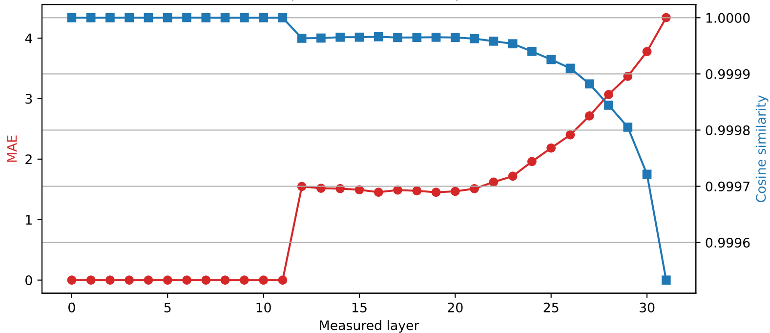
SmolLM2-360M | Quantized layer 11 | float16 \rightarrow int4
