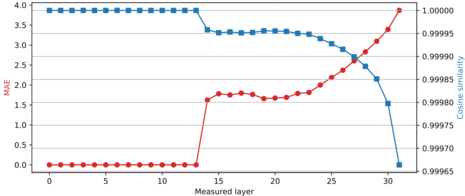
SmolLM2-360M | Quantized layer 13 | float16 → int4
