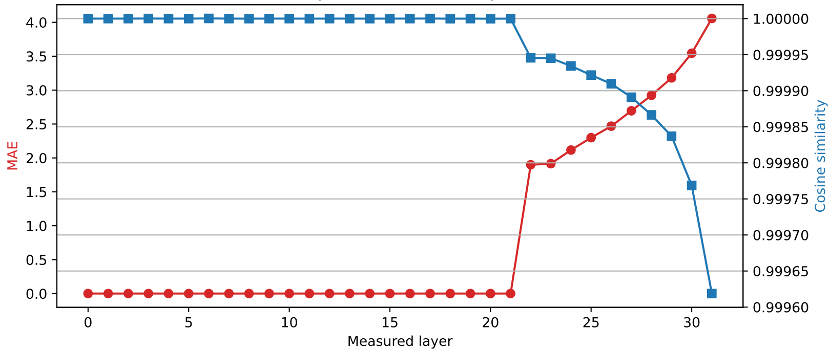
SmolLM2-360M | Quantized layer 21 | float16 → int4
