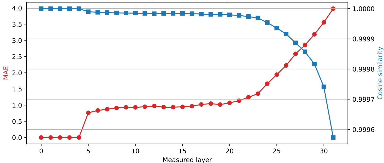
SmolLM2-360M | Quantized layer 4 | float16 → int4
