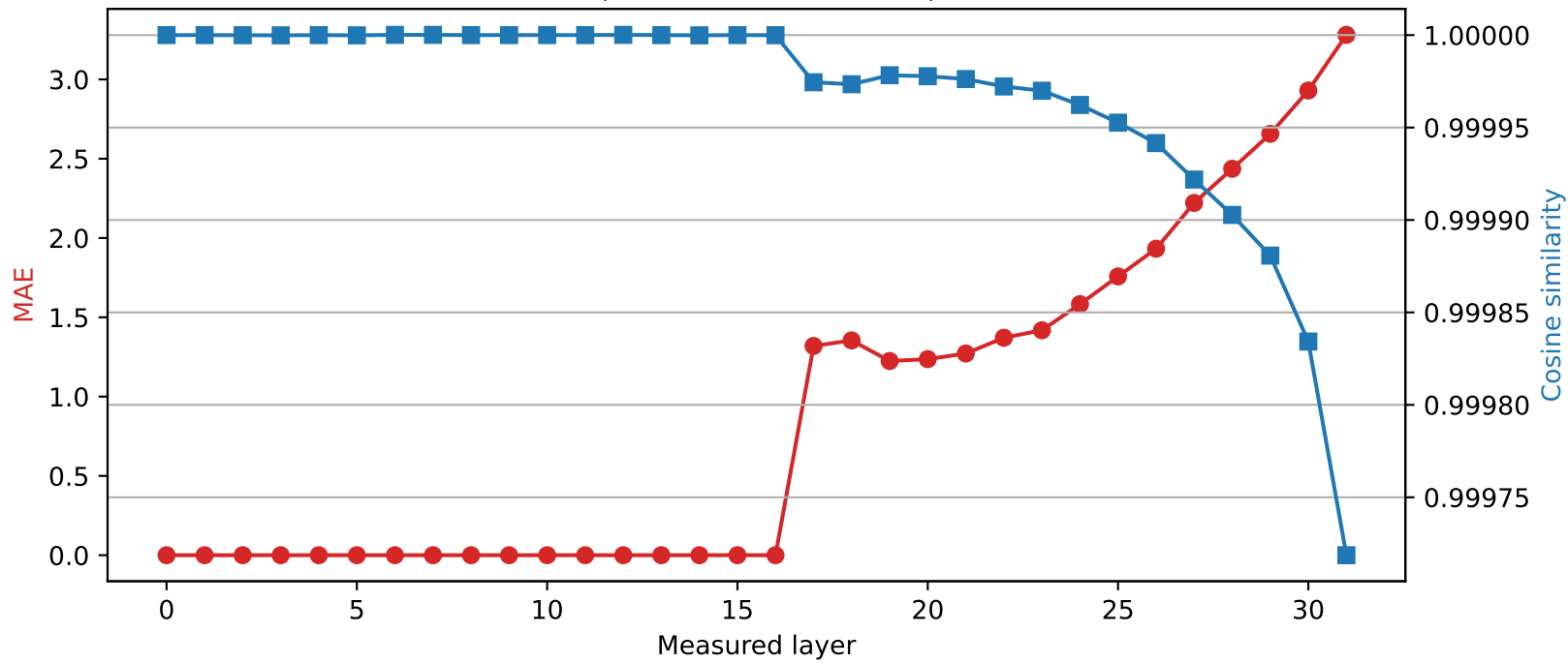
SmolLM2-360M | Quantized layer 16 | float16 → int4
