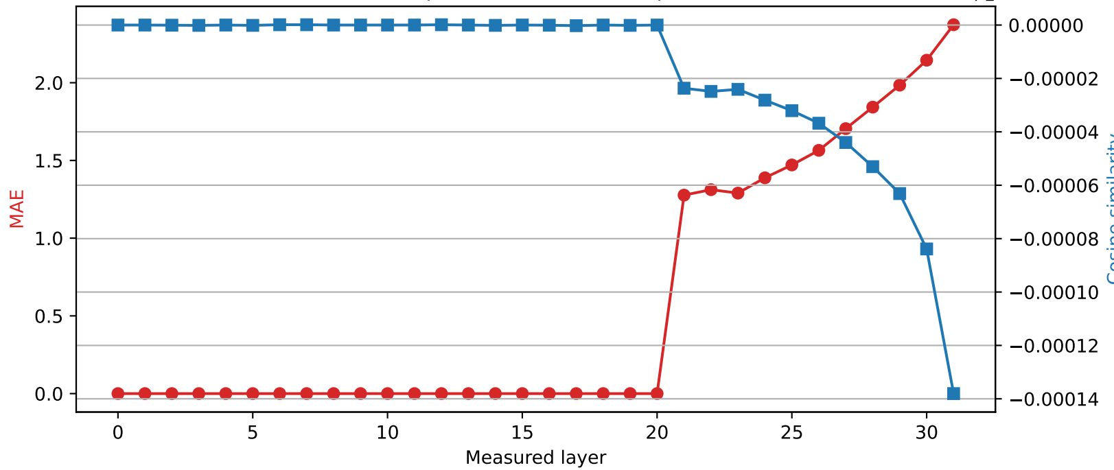
SmolLM2-360M | Quantized layer 20 | float16 \rightarrow int4
