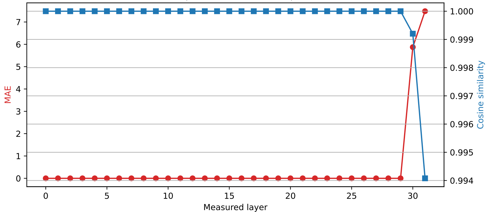
SmolLM2-360M | Quantized layer 29 | float16 \rightarrow int4
