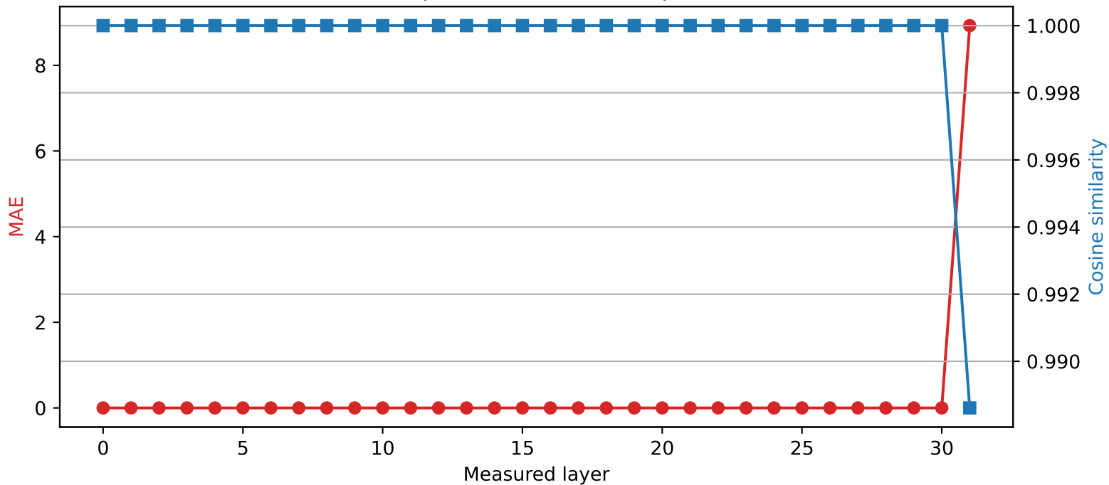
SmolLM2-360M | Quantized layer 30 | float16 \rightarrow int4
