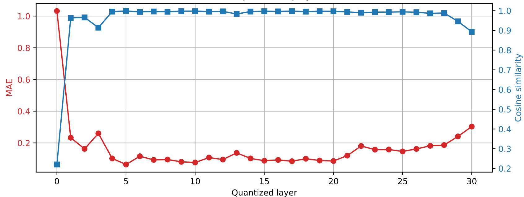
SmolLM2-360M | Prompt 4 Final RMSNorm output damage | float16 \rightarrow int4
