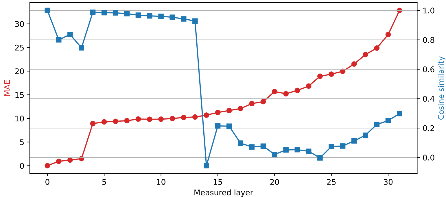
SmolLM2-360M | Quantized layer 0 | float16 \rightarrow int4
