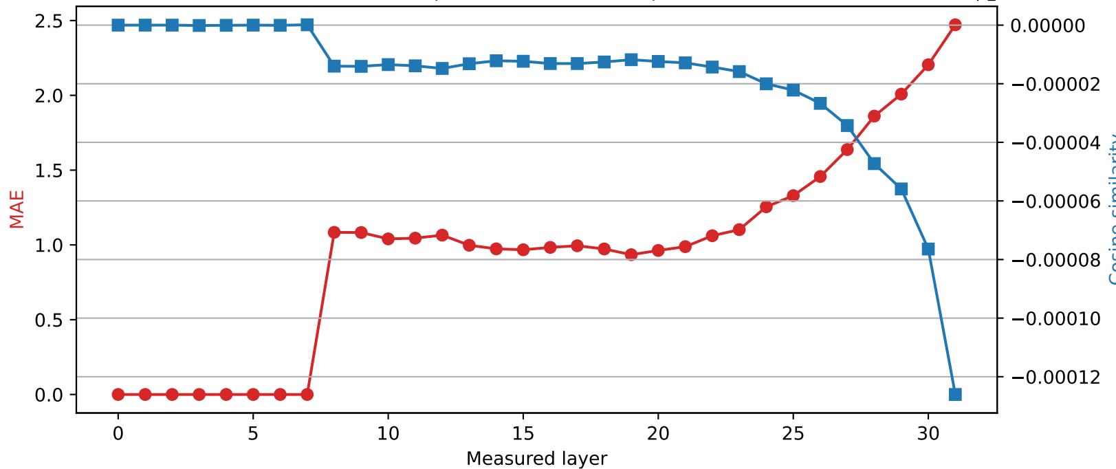
SmolLM2-360M | Quantized layer 7 | float16 → int4
