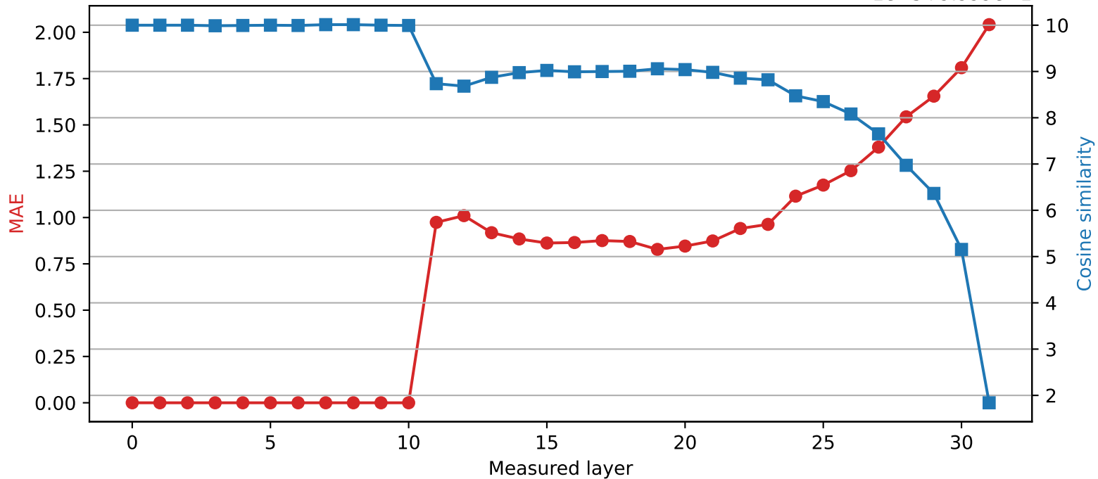
SmolLM2-360M | Quantized layer 10 | float16 \rightarrow int4 1e-5+9.999e-1
