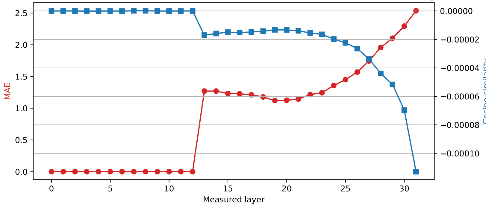
SmolLM2-360M | Quantized layer 12 | float16 → int4
