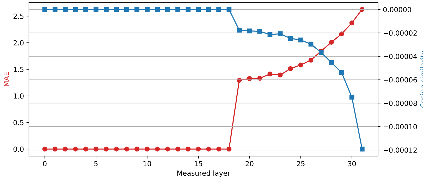
SmolLM2-360M | Quantized layer 18 | float16 → int4
