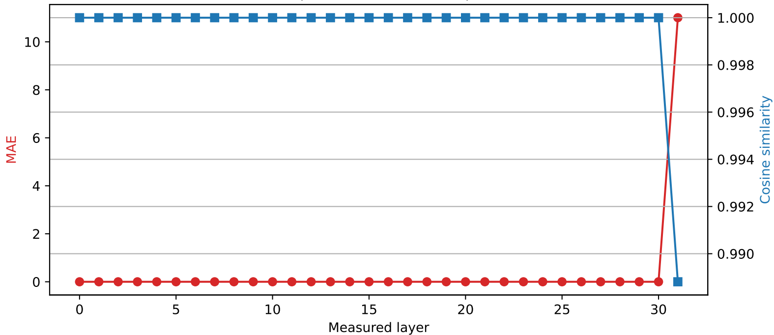
SmolLM2-360M | Quantized layer 30 | float16 → int4
