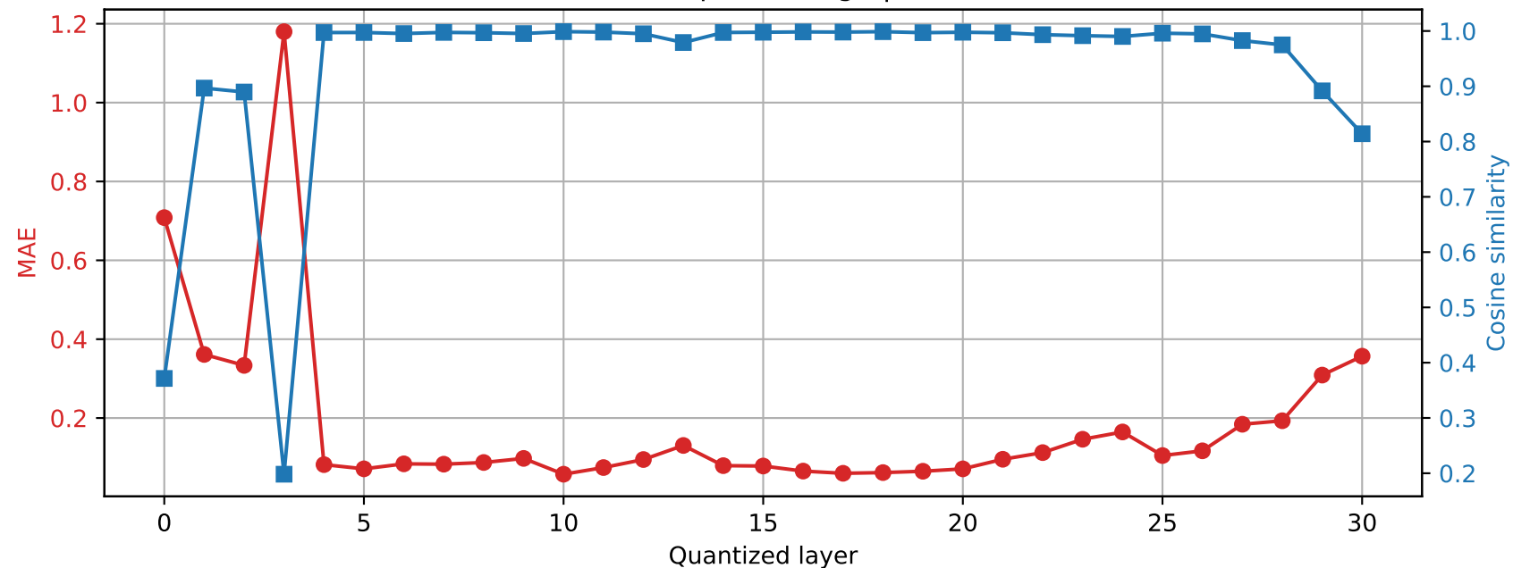
SmolLM2-360M | Prompt 0 Final RMSNorm output damage | float16 \rightarrow int2
