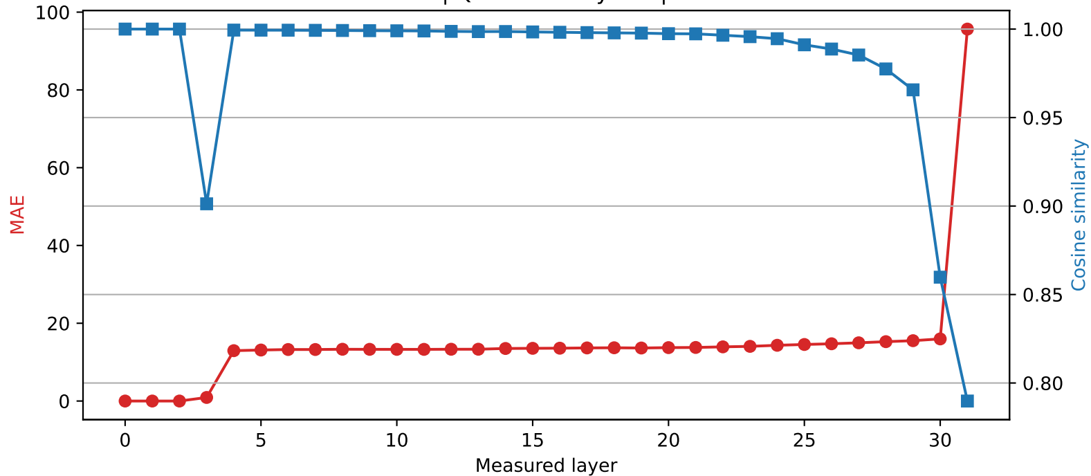
SmolLM2-360M | Quantized layer 2 | float16 \rightarrow int2
