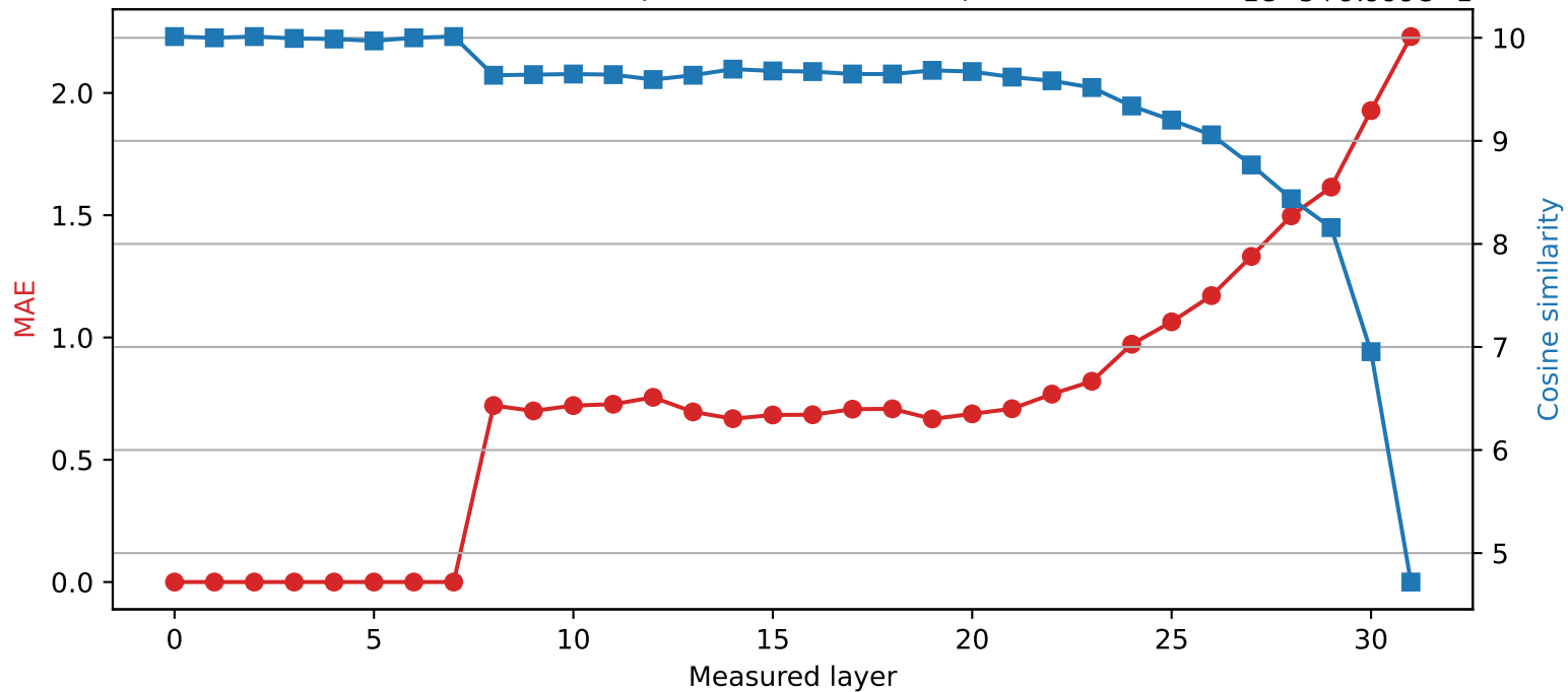
SmolLM2-360M | Quantized layer 7 | float16 → int2
