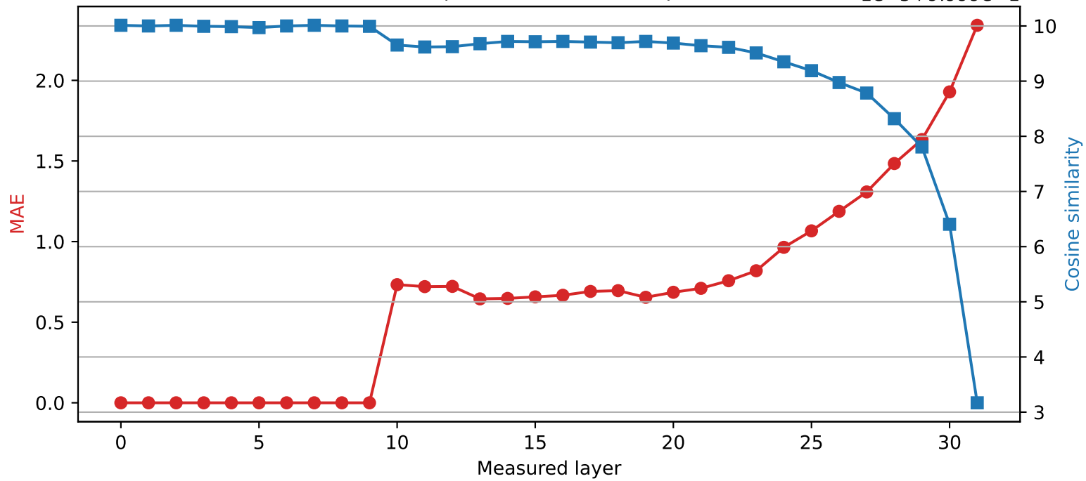
SmolLM2-360M | Quantized layer 9 | float16 → int2
