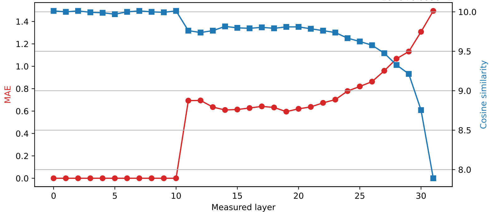
SmolLM2-360M | Quantized layer 10 | float16 → int2 1e-5+9.999e-1
