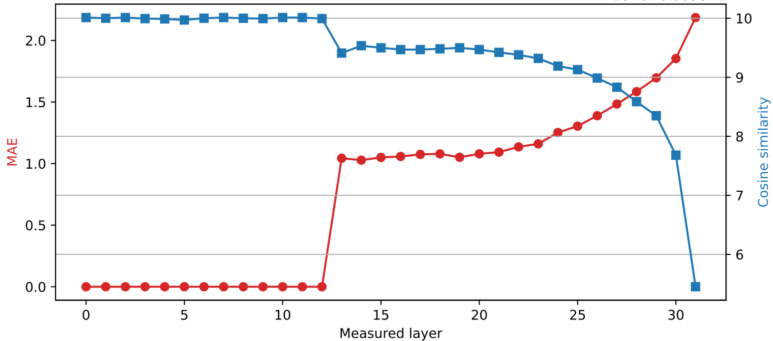
SmolLM2-360M | Quantized layer 12 | float16 → int2 1e-5+9.999e-1
