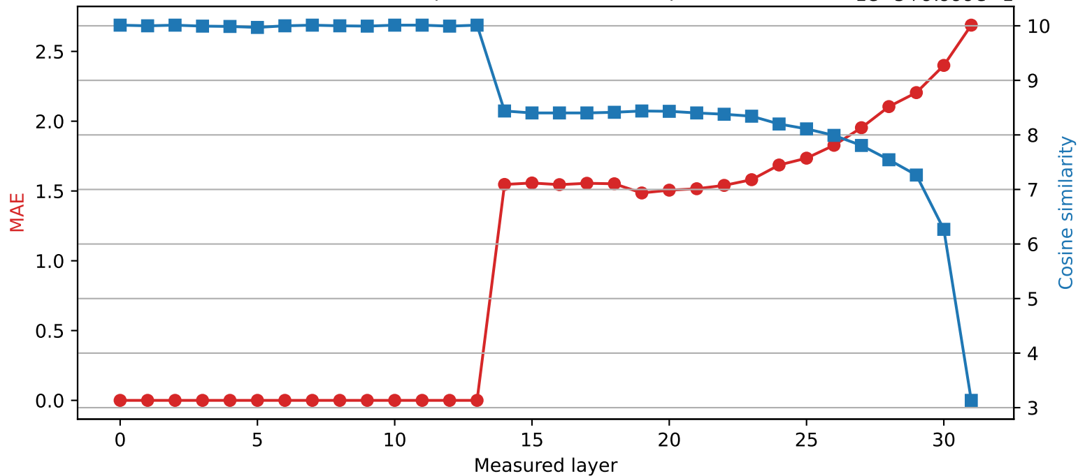
SmolLM2-360M | Quantized layer 13 | float16 → int2 1e-5+9.999e-1
