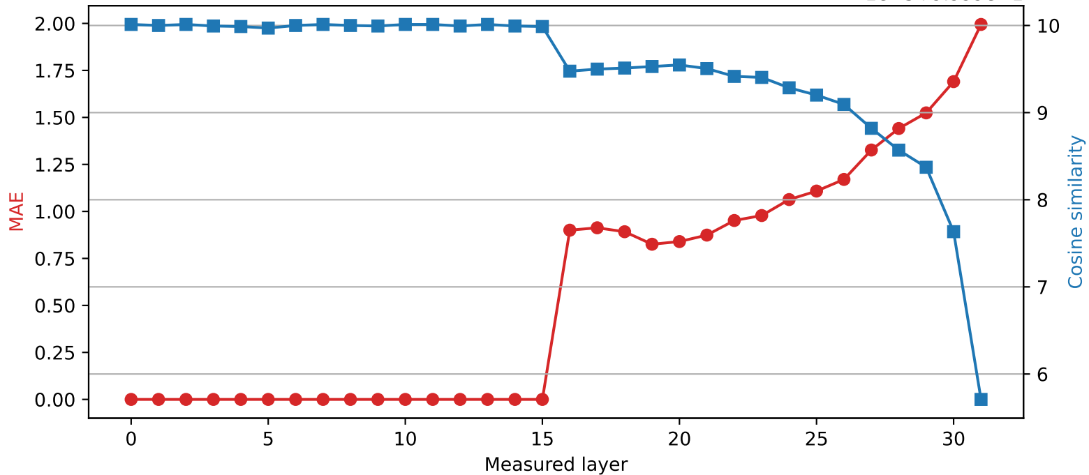
SmolLM2-360M | Quantized layer 15 | float16 \rightarrow int2 1e-5+9.999e-1
