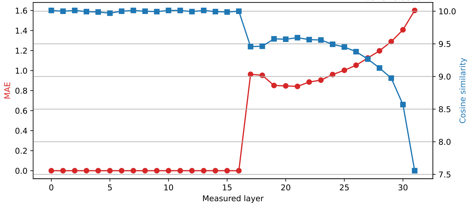
SmolLM2-360M | Quantized layer 16 | float16 → int2 1e-5 + 9.999e-1
