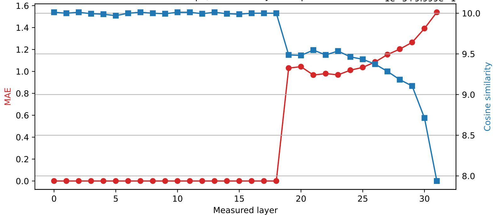
SmolLM2-360M | Quantized layer 18 | float16 \rightarrow int2 1e-5+9.999e-1
