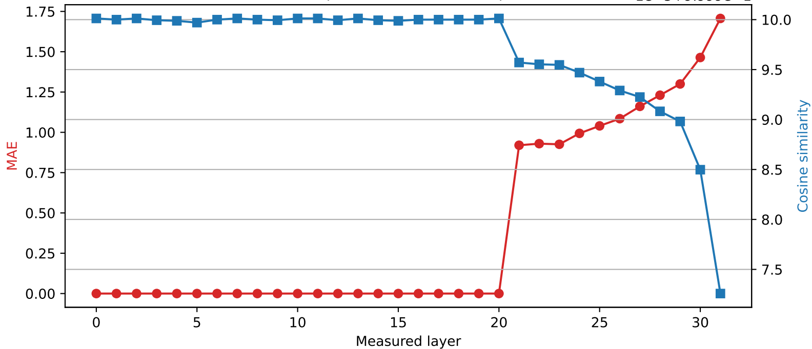
SmolLM2-360M | Quantized layer 20 | float16 → int2 1e-5+9.999e-1
