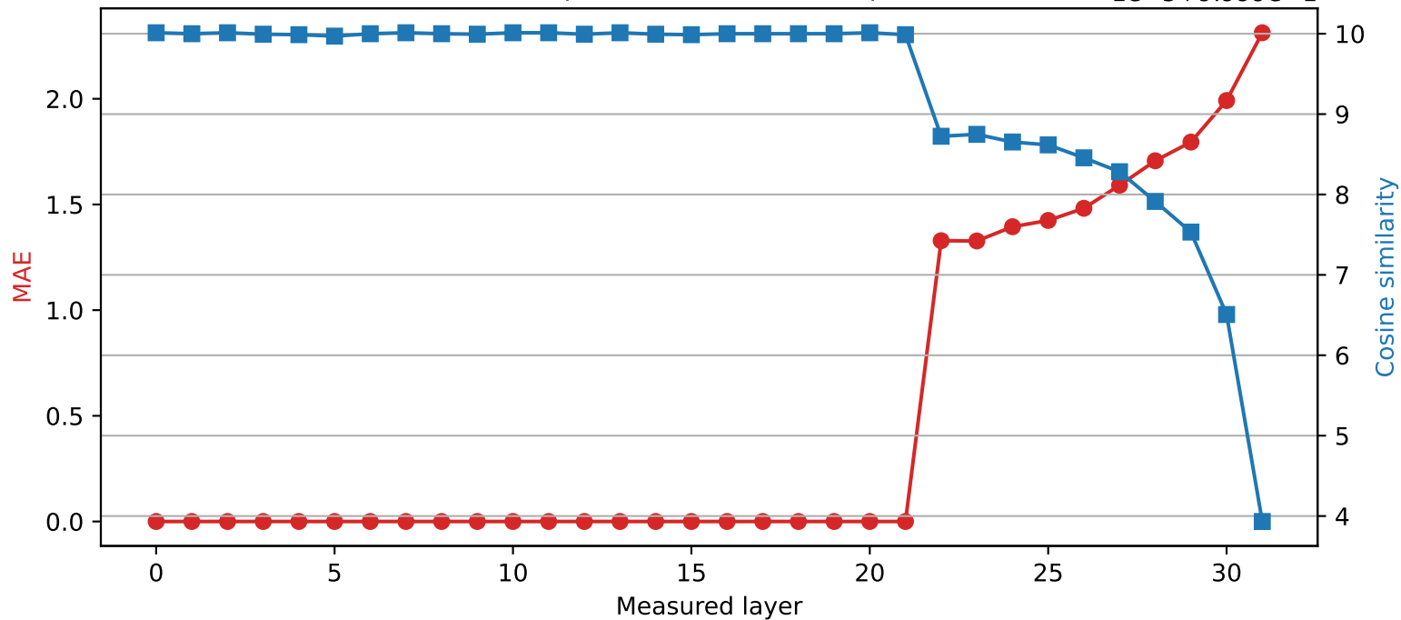
SmolLM2-360M | Quantized layer 21 | float16 \rightarrow int2 1e-5+9.999e-1
