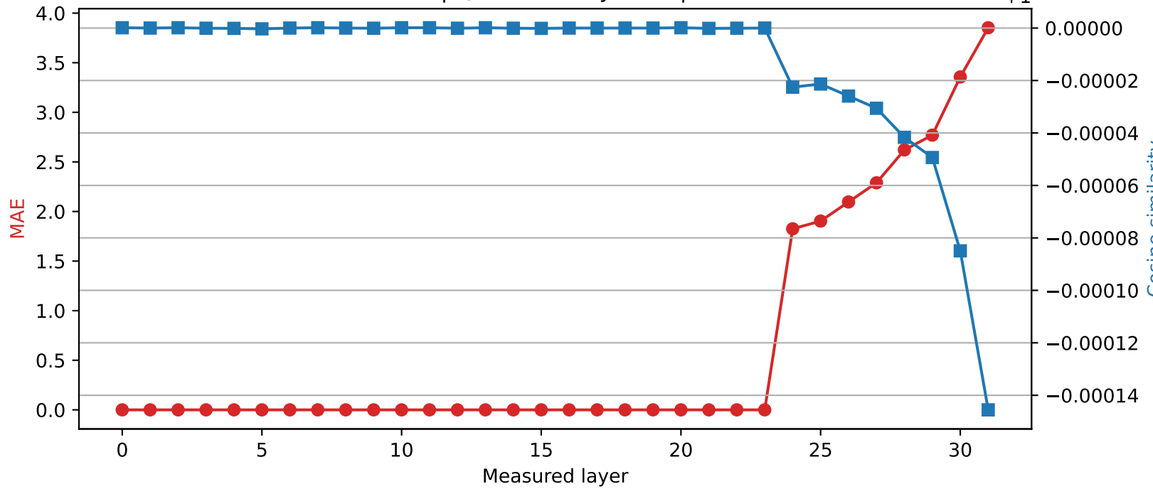
SmolLM2-360M | Quantized layer 23 | float16 → int2
