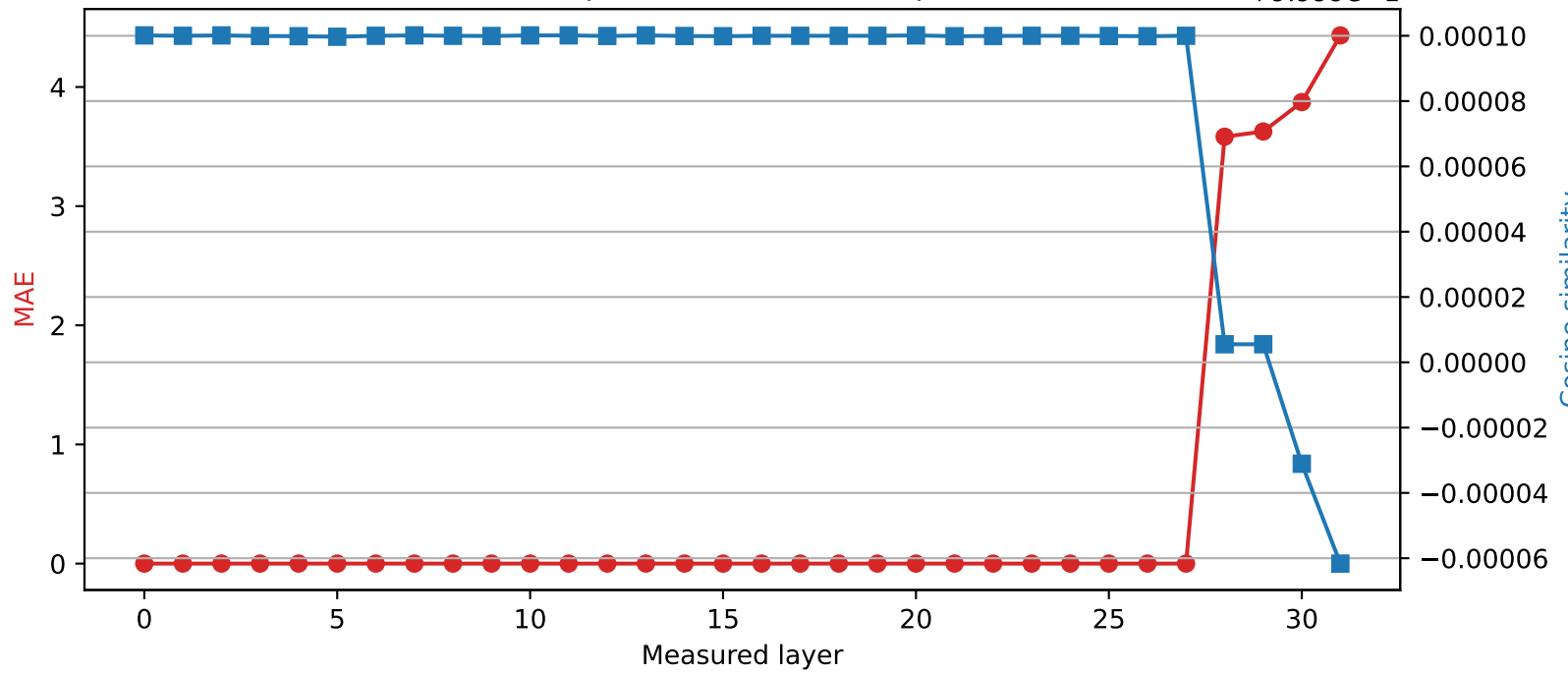
SmolLM2-360M | Quantized layer 27 | float16 → int2
