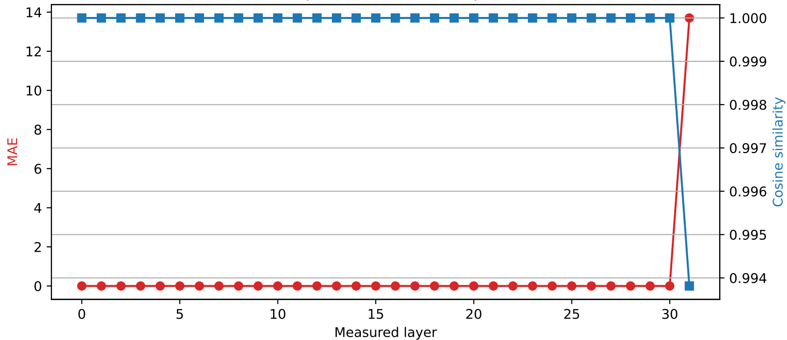
SmolLM2-360M | Quantized layer 30 | float16 \rightarrow int2
