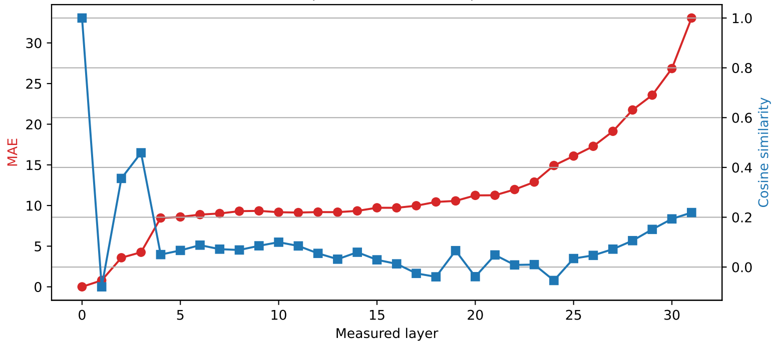
SmolLM2-360M | Quantized layer 0 | float16 → int2
