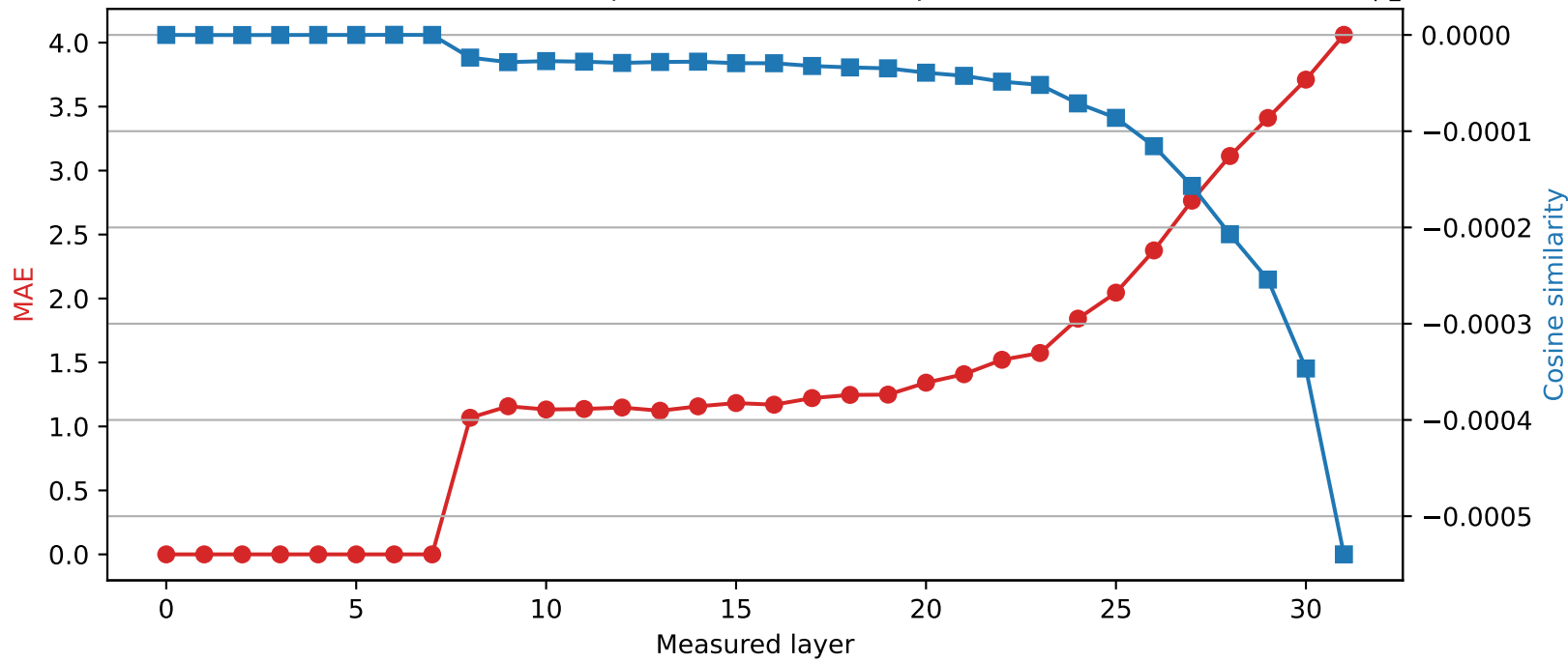
SmolLM2-360M | Quantized layer 7 | float16 \rightarrow int2
