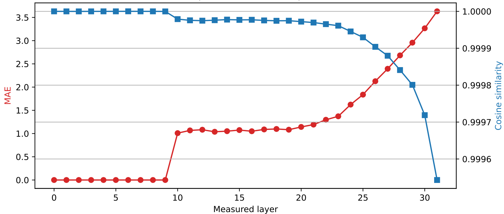
SmolLM2-360M | Quantized layer 9 | float16 \rightarrow int2
