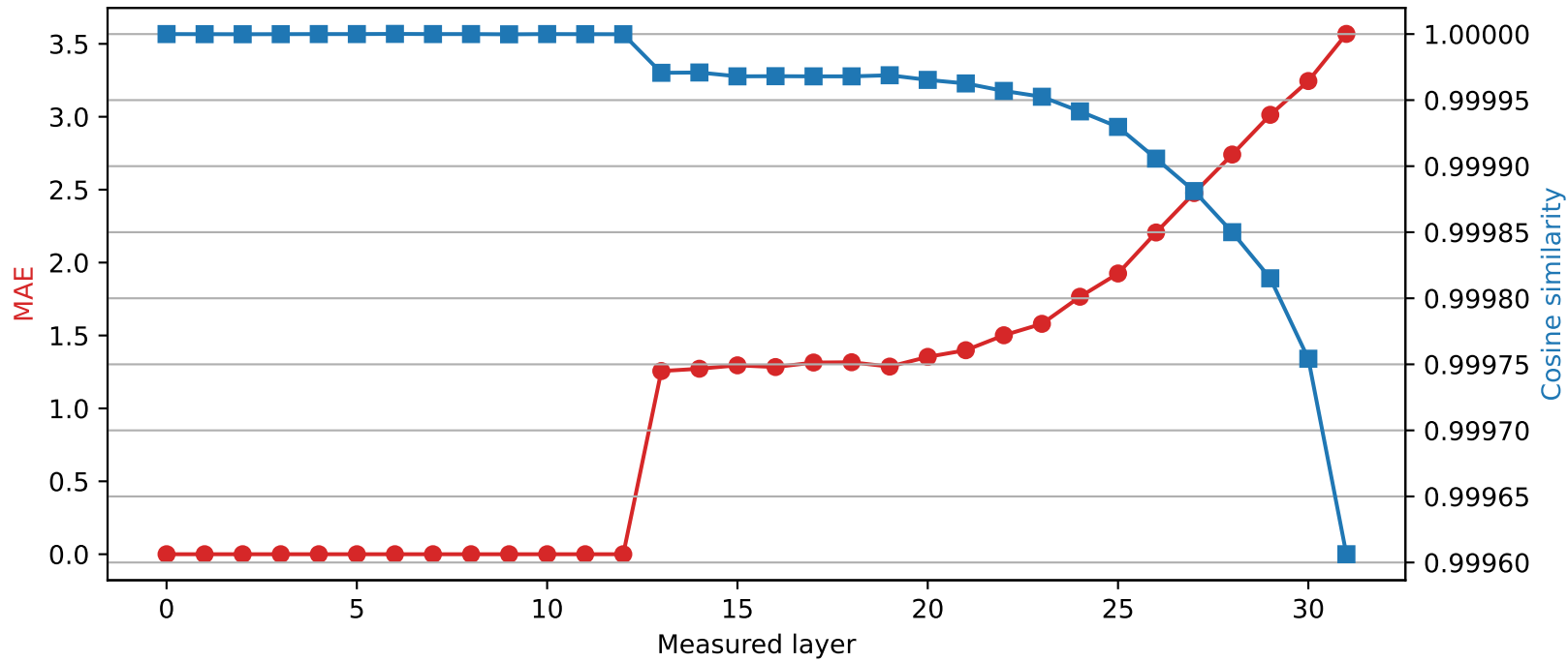
SmolLM2-360M | Quantized layer 12 | float16 → int2
