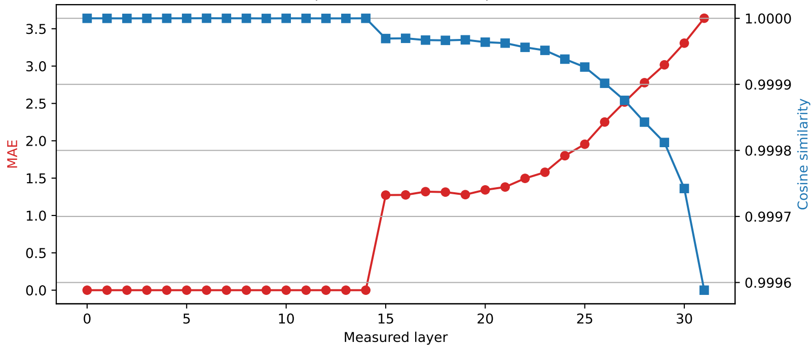
SmolLM2-360M | Quantized layer 14 | float16 → int2
