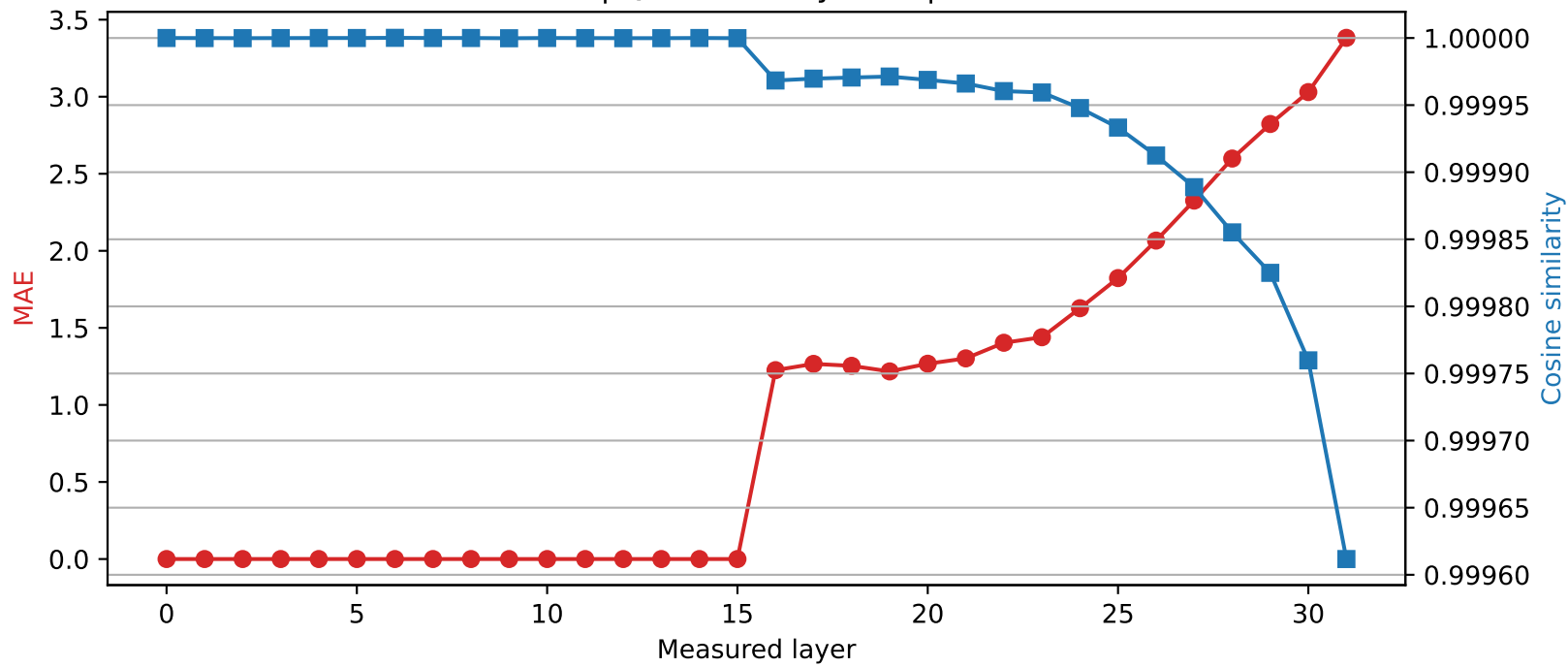
SmolLM2-360M | Quantized layer 15 | float16 \rightarrow int2
