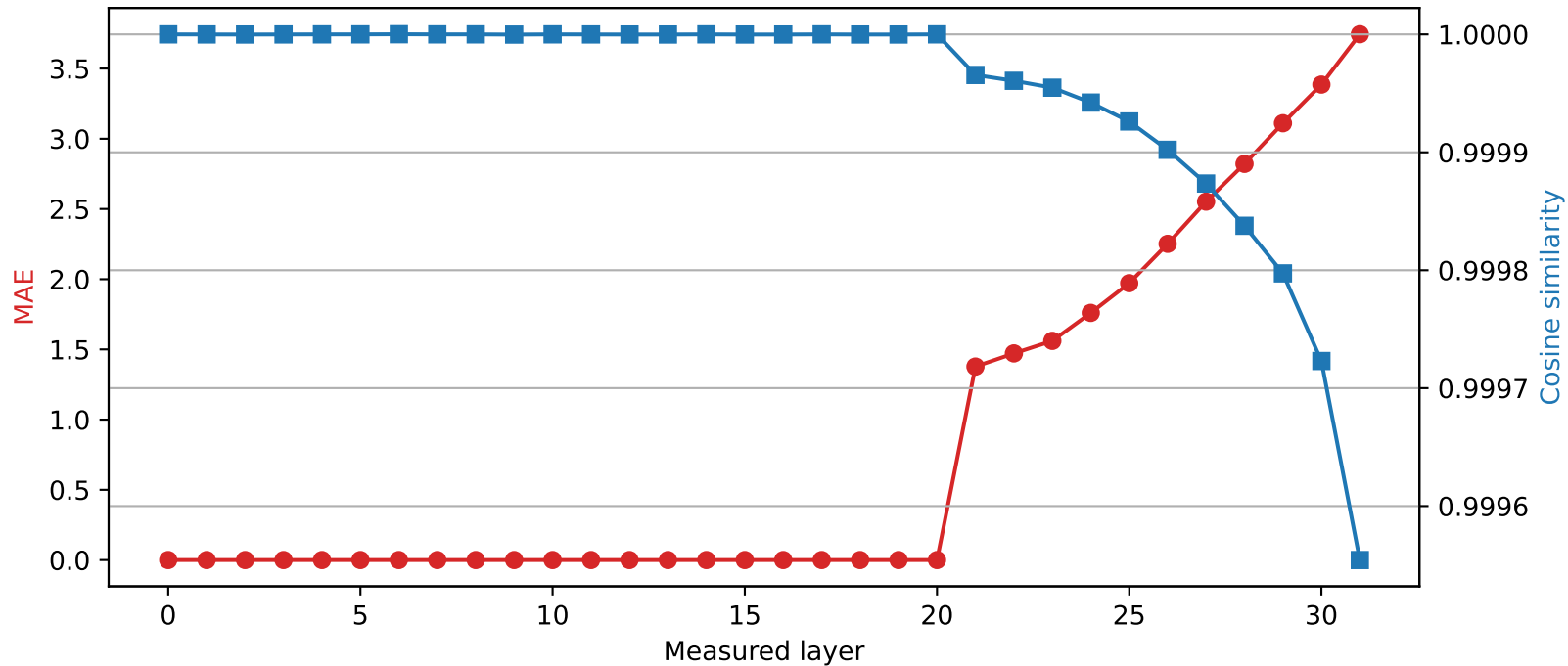
SmolLM2-360M | Quantized layer 20 | float16 → int2
