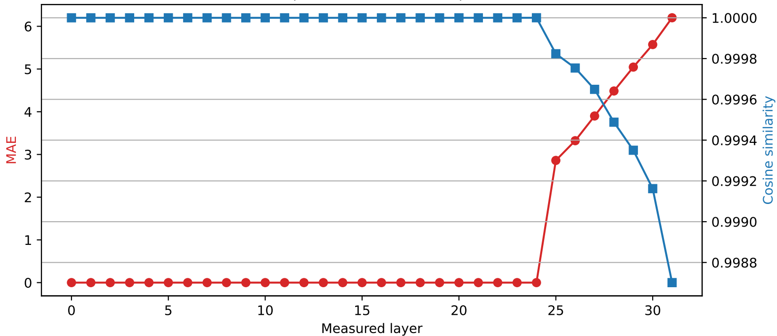
SmolLM2-360M | Quantized layer 24 | float16 \rightarrow int2
