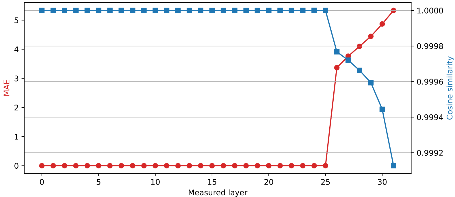
SmolLM2-360M | Quantized layer 25 | float16 \rightarrow int2
