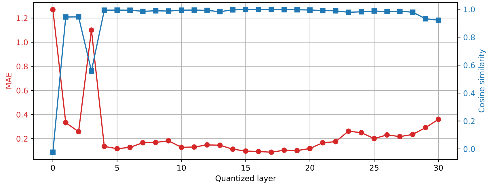
SmolLM2-360M | Prompt 2 Final RMSNorm output damage | float16 \rightarrow int2
