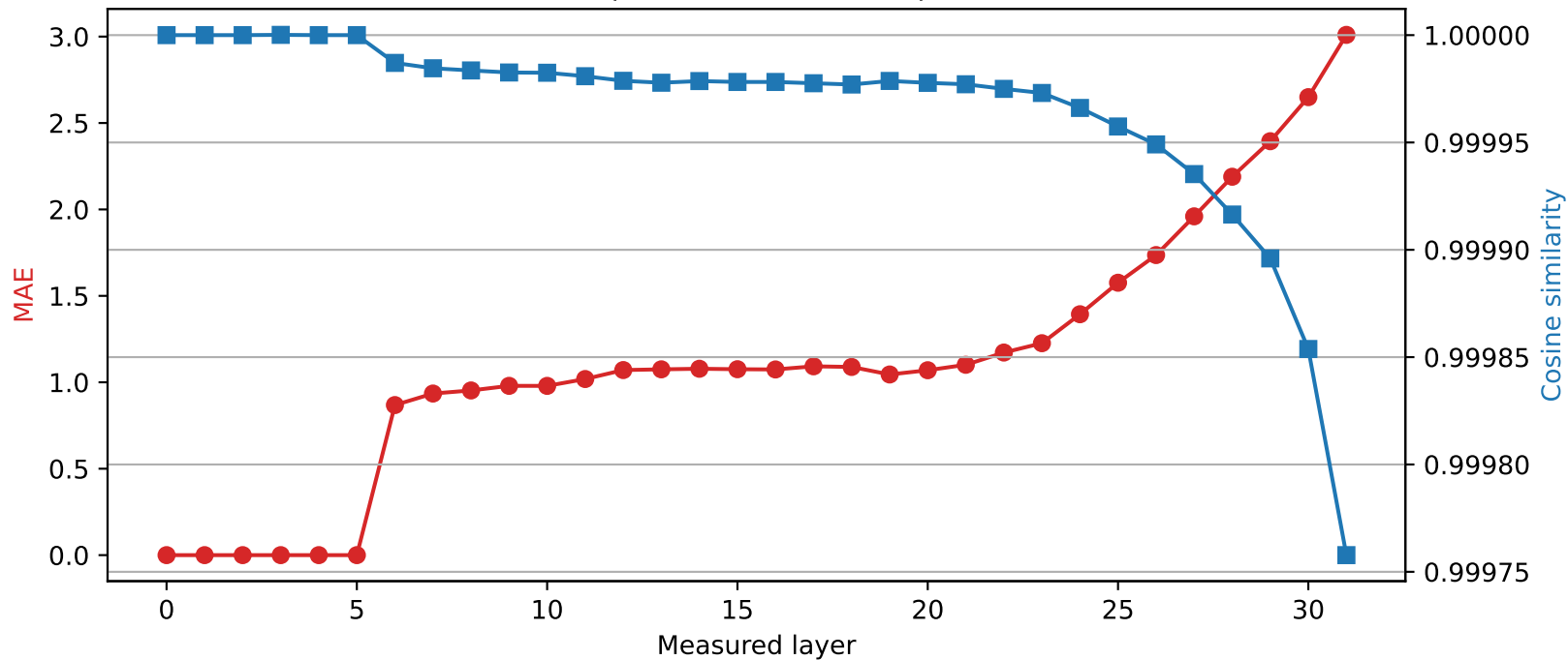
SmolLM2-360M | Quantized layer 5 | float16 \rightarrow int2
