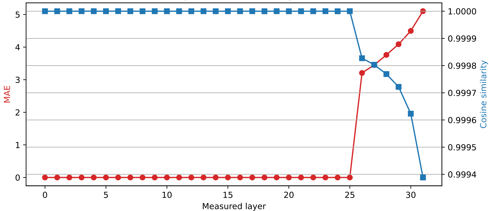
SmolLM2-360M | Quantized layer 25 | float16 → int2
