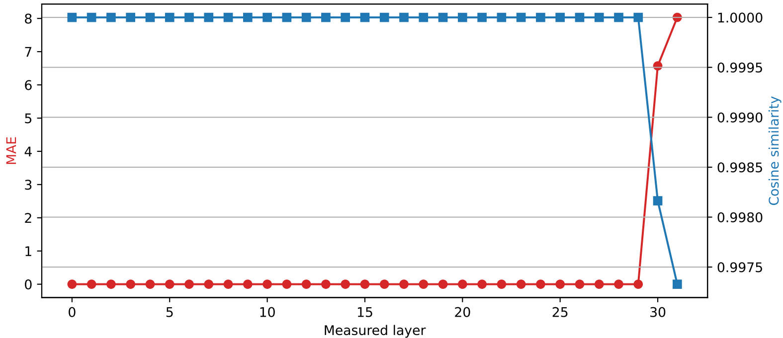
SmolLM2-360M | Quantized layer 29 | float16 \rightarrow int2
