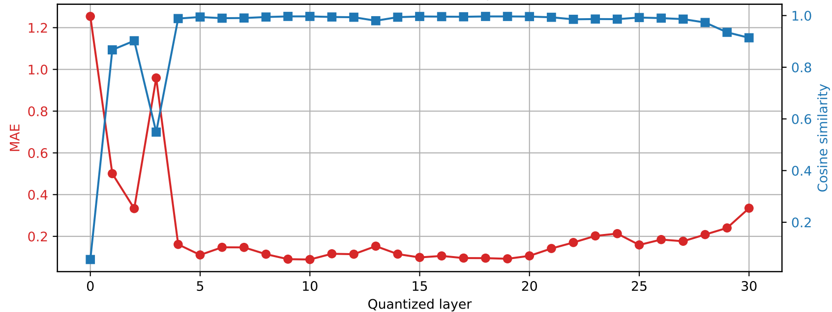
SmolLM2-360M | Prompt 3 Final RMSNorm output damage | float16 → int2
