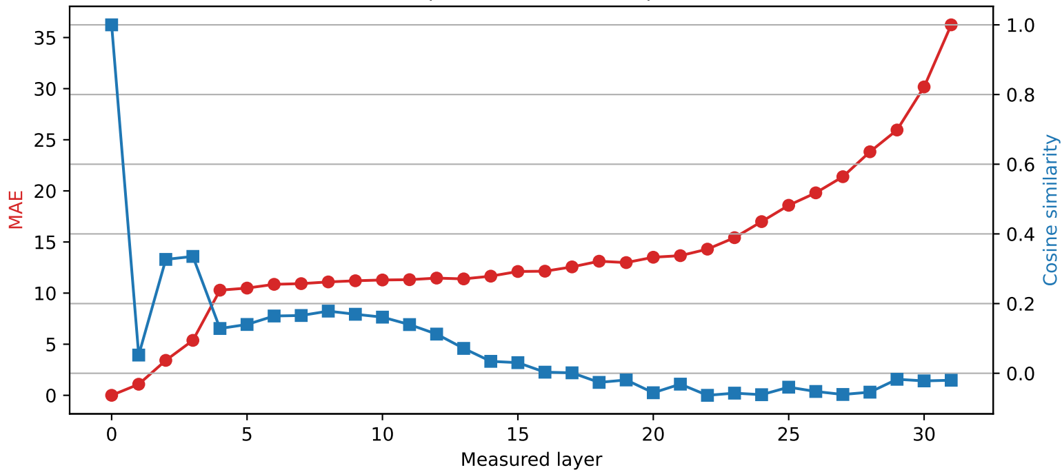
SmolLM2-360M | Quantized layer 0 | float16 \rightarrow int2
